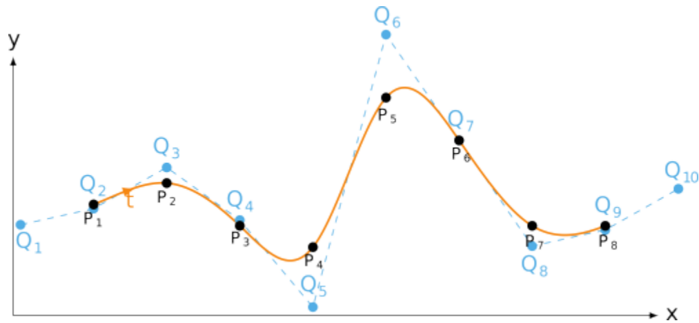
cubic spline interpolated on a set of fit knots with end-to-end tangent continuity
